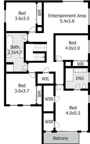
FLOOR PLAN
