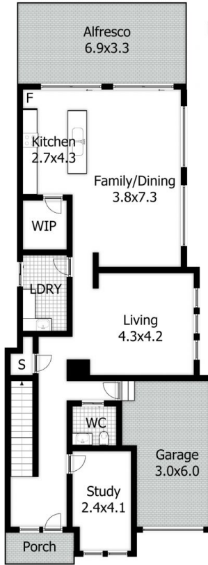
GROUND FLOOR
